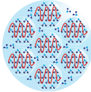
Super Coherence
